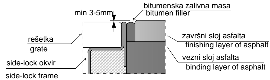
DETALJ SPOJA OKVIRA I ASFALTA DETAIL DRAWING OF JOINT BETWEEN FRAME AND ASPHALT
