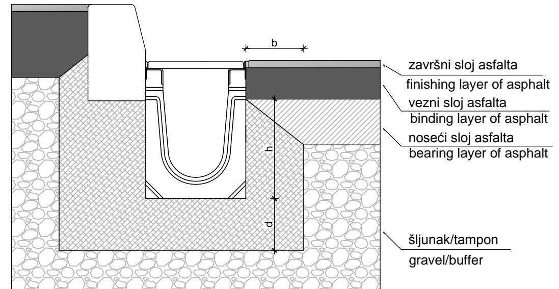
DETALJ UGRADNJE KANALETE U ASFALTNOJ POVRŠINI UZ IVIČNJAK 15/25/100 cm DETAIL DRAWING OF DRAIN CHANNEL IN ASPHALT SURFACE ALONG KERB 15/25/100 cm
