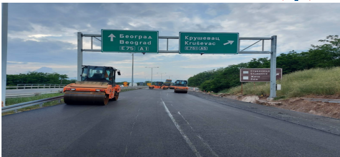
INSTALLATION OF ASPHALT LAYERS
